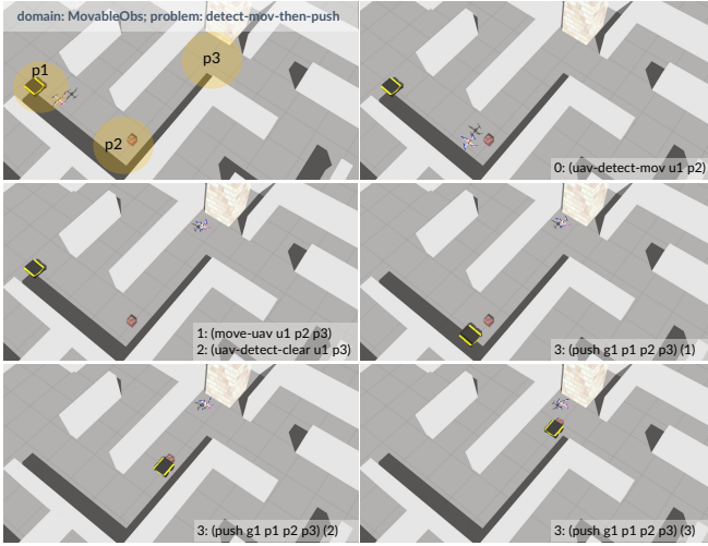
Fig. 6. Simulation of a detect-mov-then-push in the MovableObs domain. A UAV (u1) collaborates with a UGV (g1) to remove obstacles. The UAV detects a movable object at p2, verifies clearance at p3, and the UGV at p1 pushes the object from p2 to p3.
