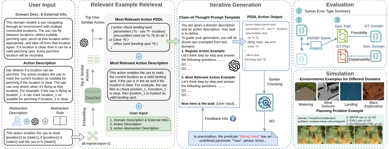
Fig. 2. The SPAR Domain Generation and Evaluation Pipeline.
