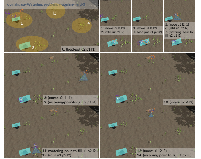
Fig. 5. Simulation of two UAVs serving four regions in the Watering domain. Example PDDL plan for watering-hard-3. UAVs u1 and u2 coordinate to load pots, move between locations, refill at water sources (I1 and I2), and perform sequential watering actions. The action watering-pour-to-fill represents pouring water to meet a location’s demand.
